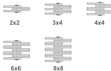
Plate lacing
